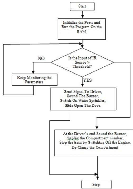
Fig 3: Flowchart of the system operation
