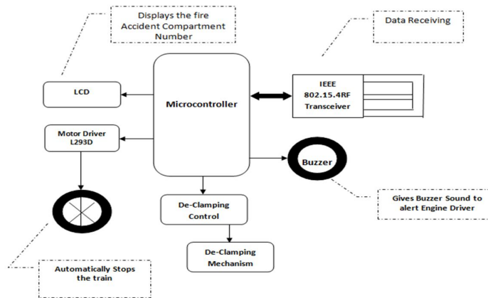
Fig 2: Block diagram of the module at the drivers end
