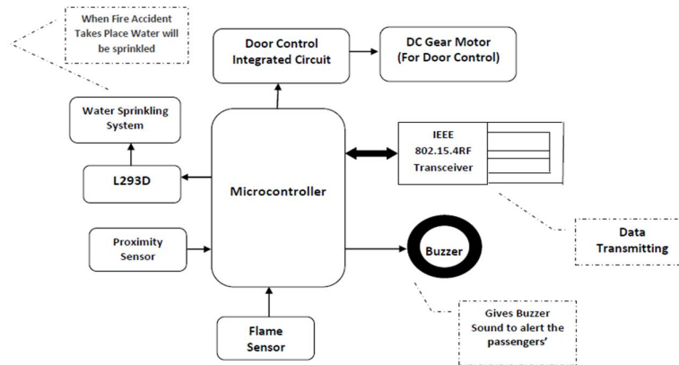
Fig 1: Block diagram of the module at the compartment
